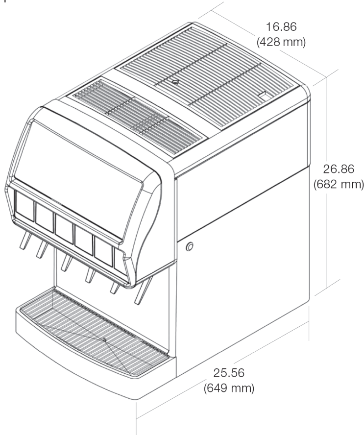
CED 600 with optional shrouded merchandiser
