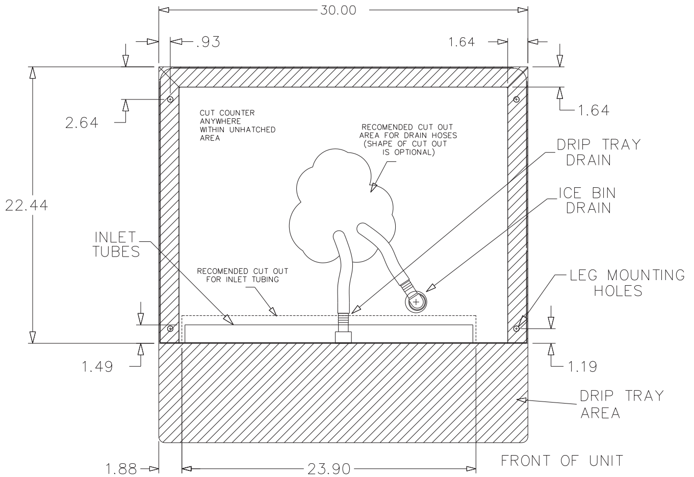
TOP VIEW OF 30" IBD FOOTPRINT (8 VALVES)
