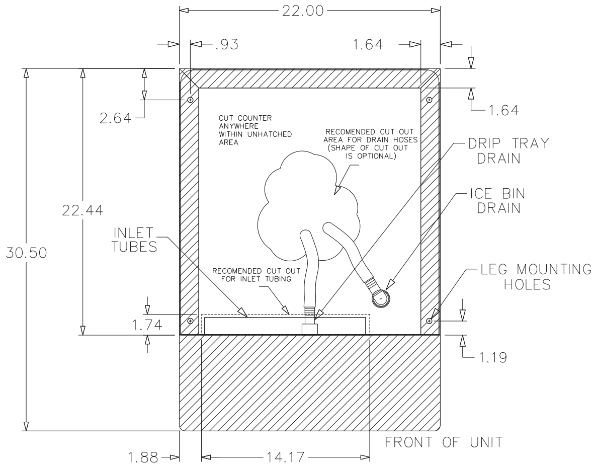
TOP VIEW OF IBD22 FOOTPRINT (6 VALVES)
