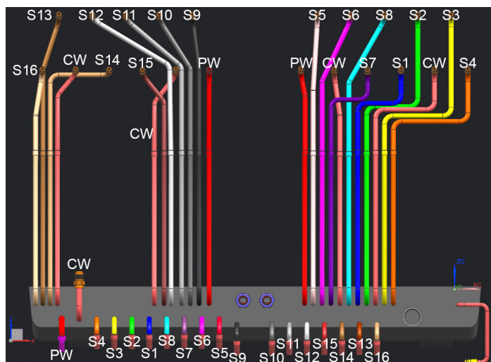
New Cold Plate Assembly, PN: 09-0338
