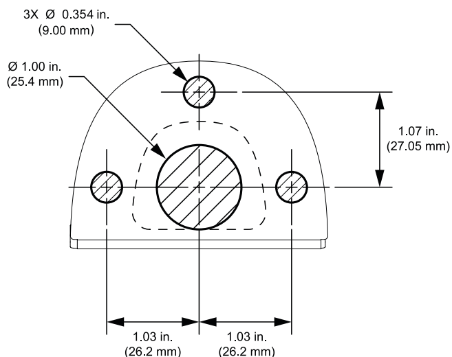
Counter Cutout For ADA Panel
