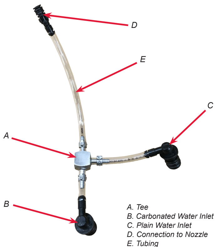
New Plumbing Assembly (Lancer PN: 49-0351)
