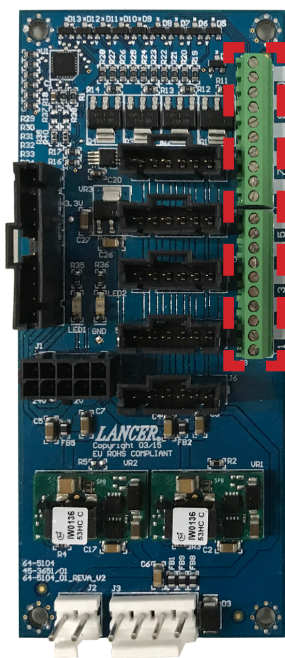
Sold Out Inputs on right side of Power PCB
